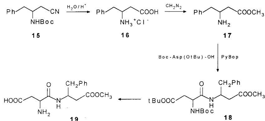
Scheme 3
